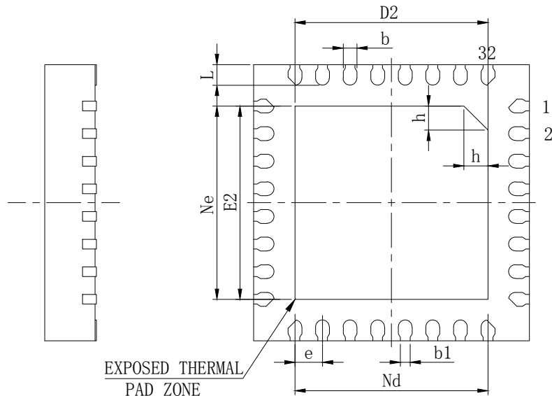
BOTTOM VIEW
