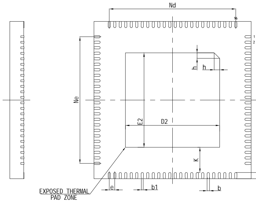
BOTTOM VIEW
