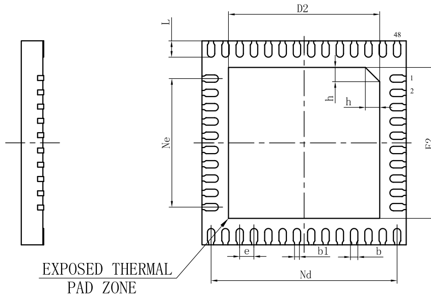
BOTTOM VIEW
