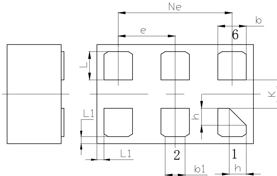
BOTTOM VIEW
