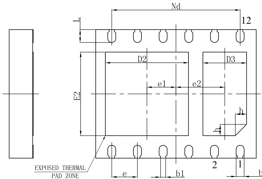
BOTTOM VIEW
