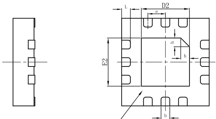
BOTTOM VIEW
