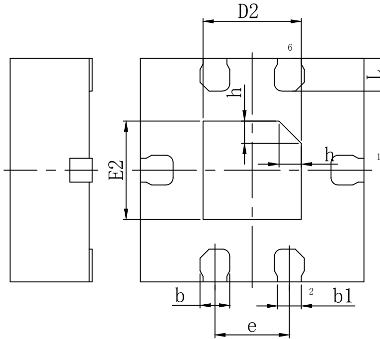
BOTTOM VIEW
